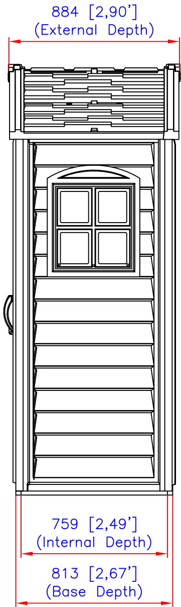
Side View
