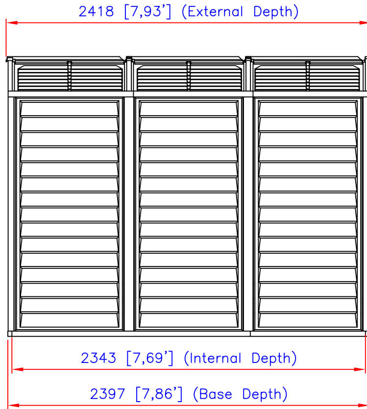
Side View
