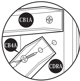
Fig. 1: Use (S1) screw. Fix (CB4A) to (CDRA)
