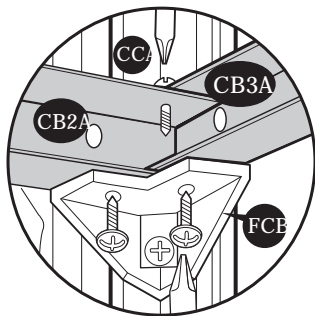
Fig. 2: Detach (CB3A) from (CB2A). Then detach (CB3A) & (CB2A) from (FCB).
