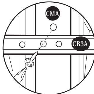
Fig.4: Use (S1) screws. Fix (CB3A) to (CMA) columns.
