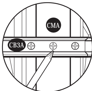
Fig.3: Fix to (CMA) with (S1) screw.
