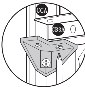
Fig.5: Use (S1) Screws. Fix (CB3A) to (FCB) fitting.
