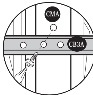
Fig. 3: Detach (CB3A) from (CMA).
