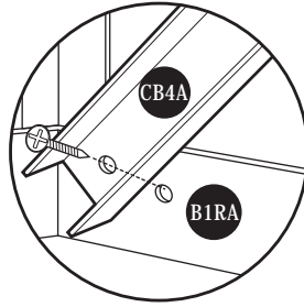
Fig. 2: Use (S1) screw. Fix (CB4A) to base (B1RA)
