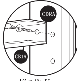
Fig. 3: Use (S1) screw. Fix (CB1A) to (CDRA)
