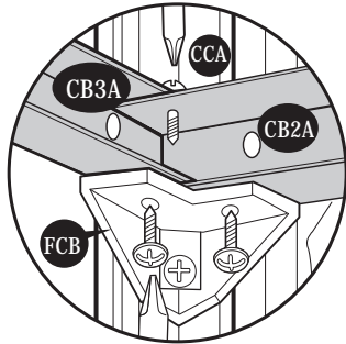
Fig. 1: Detach (CB3A) from (CB2A). Then detach (CB3A) & (CB2A) from (FCB).
