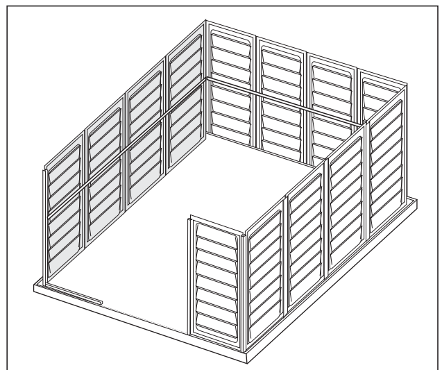
Fig.5: Use (S1) Screws. Fix (CB3A) to (FCB) fitting.
