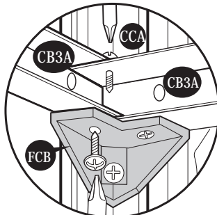
Fig.2: Use (S1) screws. Fix (CB3A) to (FCB) and (CB3A)
